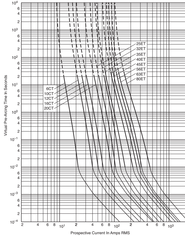
Time-Current Curve
