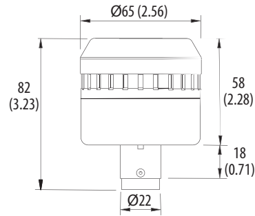
65 mm LED 65 mm Strobe
