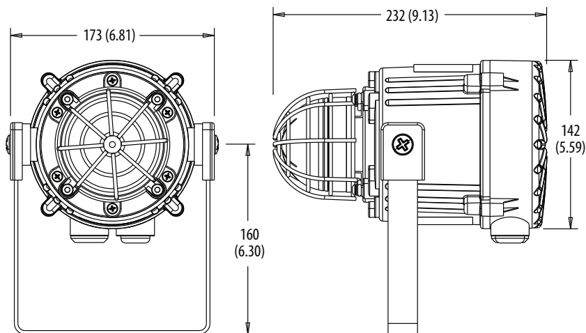
Figure 18 - Bulletin 855XB Beacons
