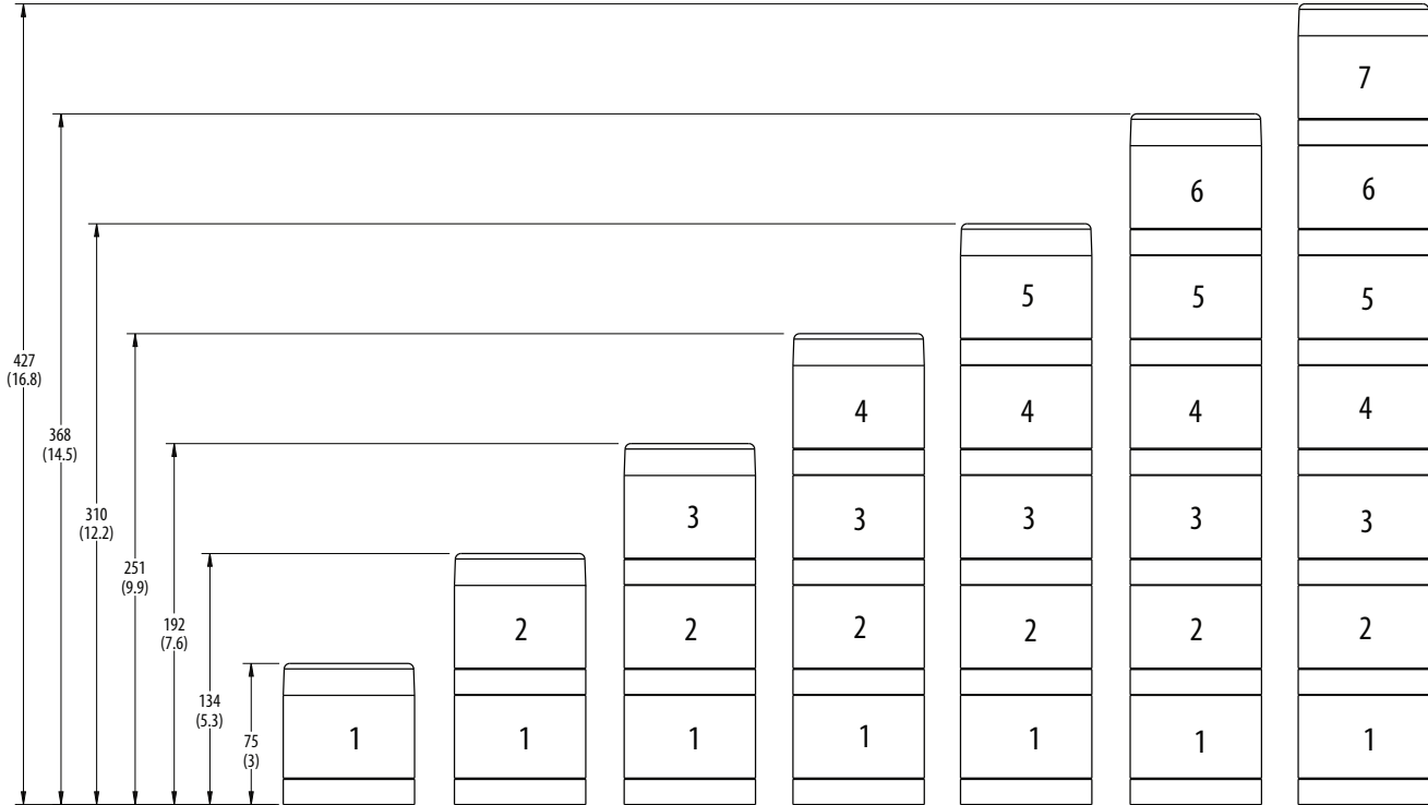
Figure 15 - Component and Accessory Dimensions
