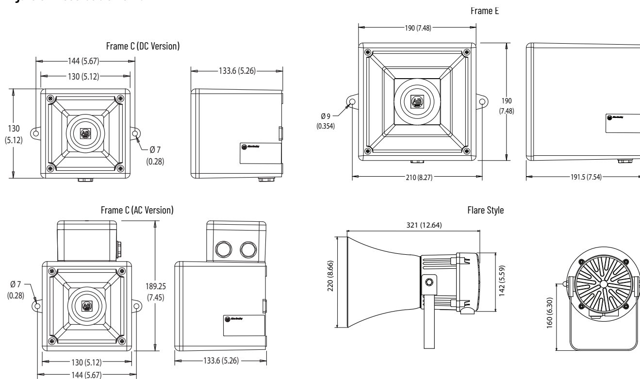
Figure 3 - Recordable Horns
