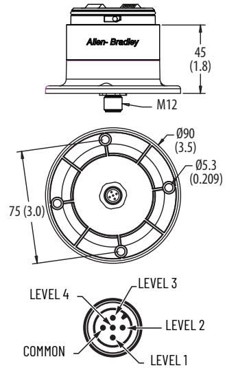
5-pin DC Micro Configuration
