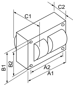
MH BAL 70W M98/143 120/277/347V KIT
