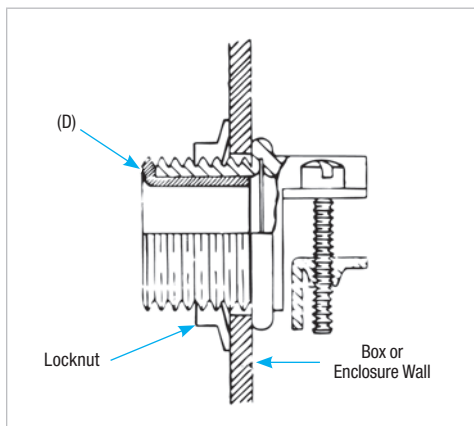
Typical Installation
