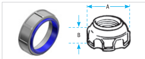
Nylon insulated metallic bushings
