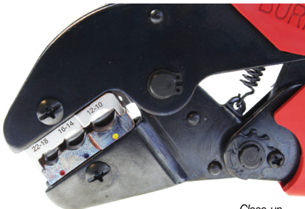
Close-up MRE1022NV
